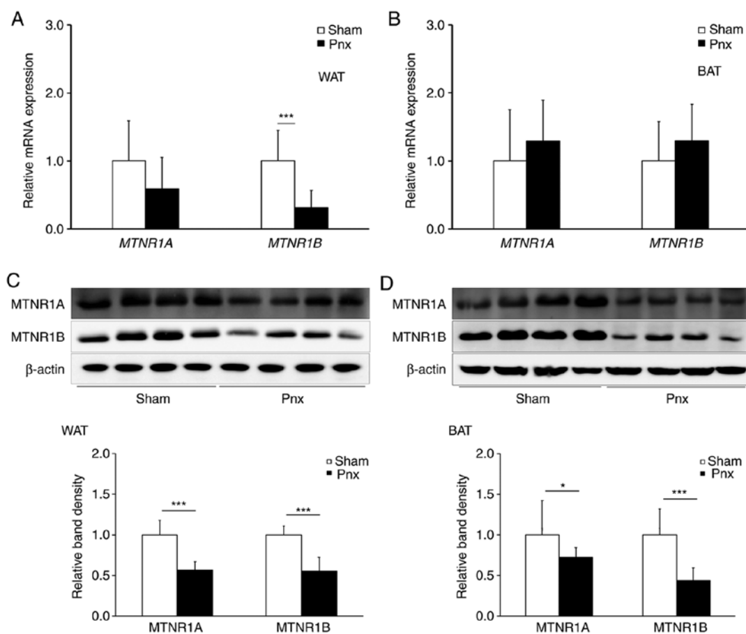
Figure 2. Expression of MTNR1A and MTNR1B in WAT and BAT. mRNA expression levels of MTNR1A and MTNR1B in (A) WAT and (B) BAT were examined by reverse transcription-quantitative PCR and normalized to \beta -actin. Protein expression levels of MTNR1A and MTNR1B in (C) WAT and (D) BAT were examined by western blotting. Values are presented as the mean \pm SD. * P < 0.05 , *** P < 0.001 vs. the sham group. Pnx, pinealectomy; WAT, white adipose tissue; BAT, brown adipose tissue; MTNR, melatonin receptor.
