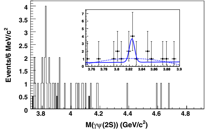
FIG. 2 (color online). The \gamma_l \psi(2S) invariant mass distribution. The open histogram is from the \psi(2S) signal mass region; the shaded histogram is from the normalized \psi(2S) mass sidebands. In the inset, the solid curve is the best fit between 3.75 \text{ GeV}/c^2 and 3.90 \text{ GeV}/c^2 and the dashed curve is a fit with only a second-order polynomial to describe the background.
