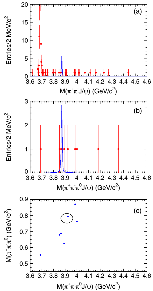
FIG. 4 (color online). (a) Distribution of the \pi^+ \pi^- J/\psi invariant mass for Y(2S) \rightarrow \gamma_R \pi^+ \pi^- J/\psi candidates. (b) Distribution of the \pi^+ \pi^- \pi^0 J/\psi invariant mass for Y(2S) \rightarrow \gamma_R \pi^+ \pi^- \pi^0 J/\psi candidates. (c) Scatter plots of m(\pi^+ \pi^- \pi^0 J/\psi) versus m(\pi^+ \pi^- \pi^0) , where the region indicated by the ellipse corresponds to the \pm 3\sigma mass regions of m(\pi^+ \pi^- \pi^0 J/\psi) and m(\pi^+ \pi^- \pi^0) from the X(3915) \rightarrow \omega J/\psi decay. Points with error bars are data; open histograms are the MC expectation for the X(3872) signal (arbitrary normalization). The peak at 3.686 \text{GeV}/c^2 in (a) is due to \psi(2S) production via ISR.
