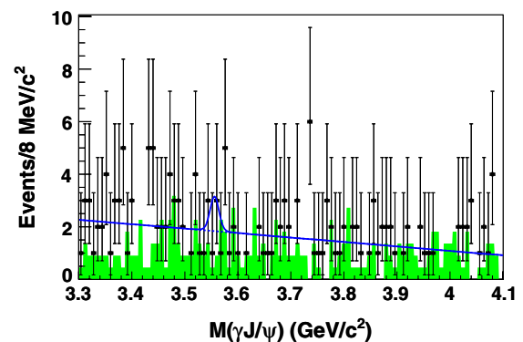
FIG. 1 (color online). The \gamma_l J/\psi invariant mass distribution. There is no \chi_{c0} , \chi_{c1} , or \chi_{c2} signal observed. The solid curve is the best fit, the dashed curve is the background, and the shaded histogram is from the normalized J/\psi mass sidebands. The signal yield is required to be non-negative in the fit.
