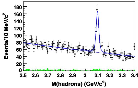
FIG. 3 (color online). The mass distribution for a sum of the five \eta_c decay modes. The solid curve is a sum of the corresponding functions obtained from a simultaneous fit to all the \eta_c decay modes, and the dashed curve is a sum of the background functions from the fit. The shaded histogram is a sum of the off-resonance events (not normalized). The J/\psi signal is produced via ISR rather than from a radiative decay of an Y(nS) resonance.
