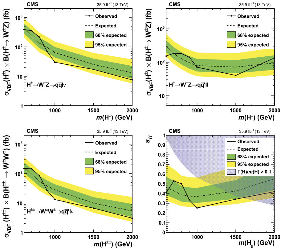
Fig. 5. Expected and observed exclusion limits at the 95% CL as a function of m(H^\pm) for \sigma_{\text{VBF}}(H^\pm)\mathcal{B}(H^\pm \rightarrow W^\pm Z) in the WV (upper left) and ZV (upper right) final states, for \sigma_{\text{VBF}}(H^{\pm\pm})\mathcal{B}(H^{\pm\pm} \rightarrow W^\pm W^\pm) , as a function of m(H^{\pm\pm}) (lower left), and for s_H in the GM model (lower right). The blue shaded area covers the theoretically disallowed parameter space [76].
