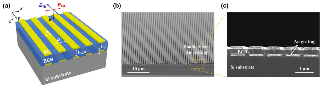
Figure 1. (a) Schematic illustration of the double-layer Au grating composed of the dielectric spacer situated between identical Au gratings. Here, p is the Au grating periodicity ( 1 \mu\text{m} ), w is the Au grating width ( 0.7 \mu\text{m} ), t_{\text{Au}} is the metal thickness ( 0.1 \mu\text{m} ), and t_{\text{BCB}} is the BCB thickness ( 0.25 \mu\text{m} ) between the gratings. (b) Tilted-view and (c) cross-sectional-view scanning electron microscope (SEM) images of the double-layer Au grating.
