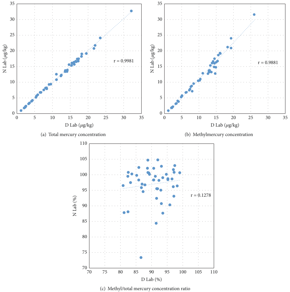
FIGURE 1: Distribution and correlation coefficient ( r value) of (a) total mercury concentration, (b) methylmercury concentration, and (c) methyl/total mercury concentration ratio between D Lab in Korea and N Lab in Japan.
