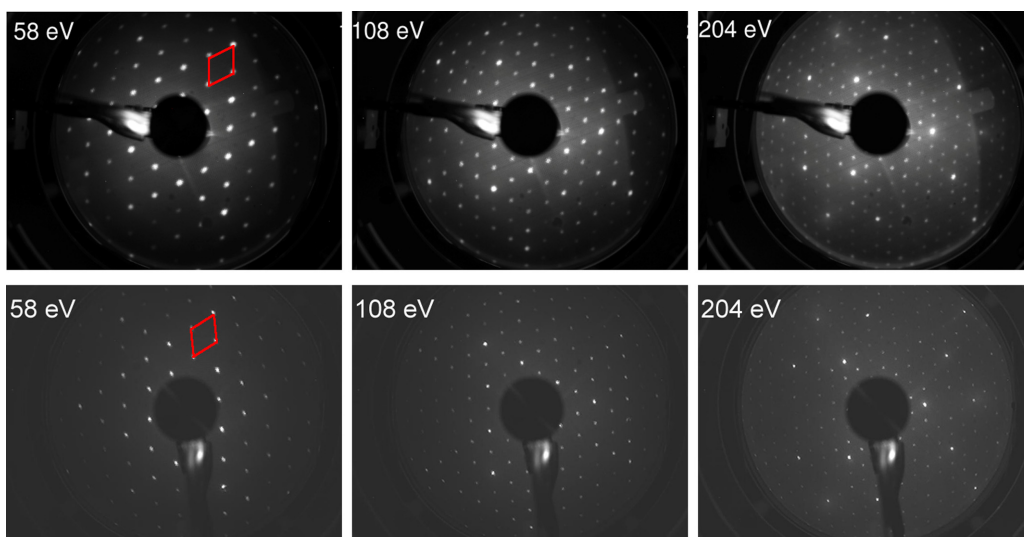
FIG. 6. LEED patterns of the B-2\sqrt{3}\text{Sn} (top) and n-2\sqrt{3}\text{Sn} (bottom) surfaces, recorded at three different beam energies and acquired at a sample temperature of 90 K. The unit cell of the reciprocal lattice is indicated in red in the two panels on the left ( 58 eV).
