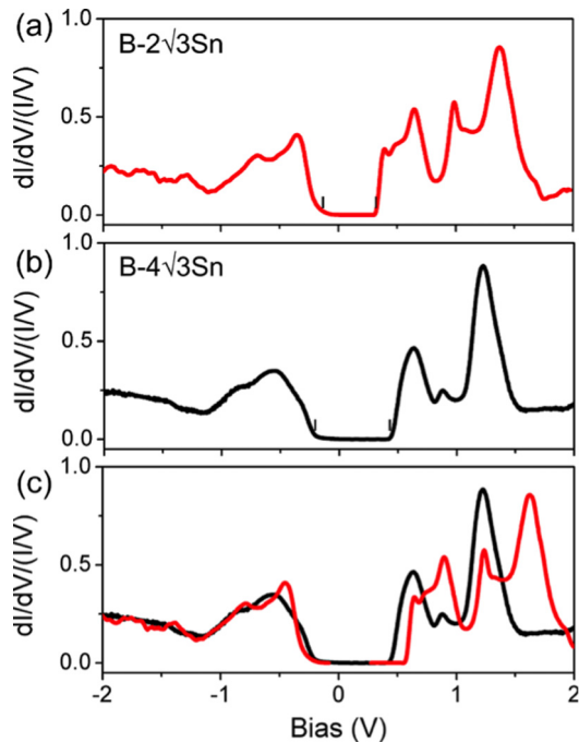
FIG. 11. Normalized dI/dV spectra of the (a) B-2\sqrt{3}\text{Sn} and (b) B-4\sqrt{3}\text{Sn} surface, measured at 4.4 K. Both spectra were recorded with the STM tip positioned above a down atom. (c) shows a line-up of the spectra after stretching the band gap in (a) (the filled states shift 0.1 V toward a lower energy, while the empty states shift 0.24 V toward a higher energy) to match the band gap value in (b). Note the absence of a peak at +1.7 V in the B-4\sqrt{3}\text{Sn} spectrum. Such a peak does exist, however, when the spectrum is recorded on the up atom (Fig. 12). The band gap values in (a) and (b) are 0.45 and 0.70 eV (marked by tick marks), respectively.
