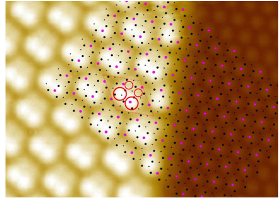
FIG. 4. STM image showing coexisting domains of the \sqrt{3} and 2\sqrt{3} reconstructions. The \sqrt{3} reconstruction consists of 1/3 ML of Sn adsorbed at the T_4 adatom sites of the Si(111) substrate. Note that there are three T_4 sites per \sqrt{3} unit cell. The grid overlay thus allows us to determine the registry of the top layer atoms of the 2\sqrt{3} reconstruction (see text). The black solid dots are the atoms of the outermost Si bilayer and the purple solid dots mark the T_4 adsorption sites. The rhombic 2\sqrt{3} -Sn unit cell is indicated. The “up” and “down” atoms of the Sn tetramer are indicated by the large and small red circles, respectively. The up atoms are approximately located at the T_4 sites while the down atoms are located above the three fold hollow ( H_3 ) sites of the Si(111) substrate.
