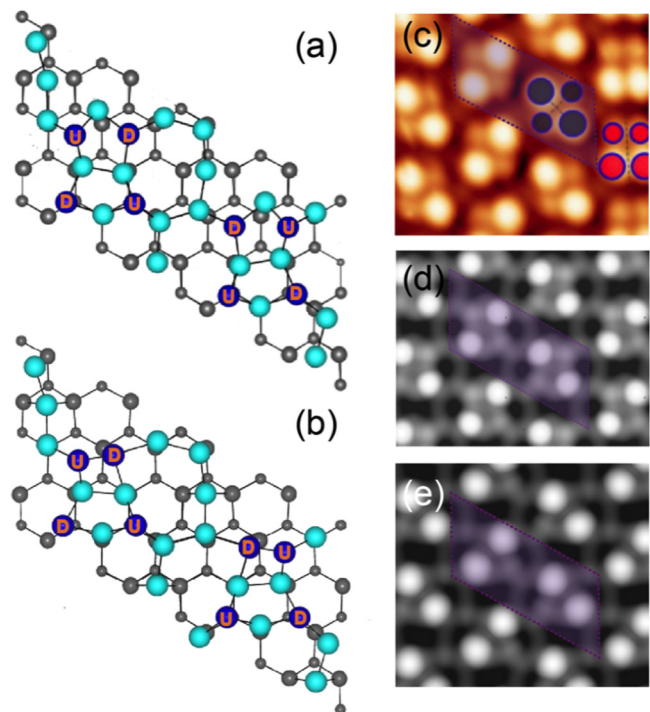
FIG. 8. Fully optimized geometry of the n-4\sqrt{3} Sn structure, starting with the optimized Törnevik coordinates (a) and revised trimer (b) coordinates. The up (U) and down (D) atoms of the Sn tetramers are indicated. (c) Empty state experimental STM image of the B-4\sqrt{3} Sn structure, scanned at +1 V, 0.2 nA. This STM image is noise filtered. Note the existence of a narrow 2\sqrt{3} strip on the far right of the image. The up atom and down atom positions are indicated by large and small filled circles, respectively (dark blue for the 4\sqrt{3} structure and red for the 2\sqrt{3} structure). Simulated empty state STM images of the 4\sqrt{3} structures based on the Törnevik (d) and revised trimer (e) models, all at +1 V bias voltage. The purple shaded parallelograms mark the (4\sqrt{3} \times 2\sqrt{3})R30^\circ unit cell.
