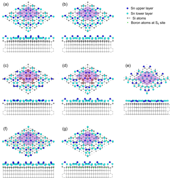
FIG. 3. Top view and side view of the total-energy-minimized geometry of the 2\sqrt{3} -Sn structure for (a) the Törnevik model [18]; (b) the revised Törnevik model; (c) trimer model; (d) revised trimer model; and (e) Ichikawa model [21]. The encircled Sn atoms in (c) and (d) are the original trimer atoms of the 2\sqrt{3} * structure prior to the DFT structure optimization of the 2\sqrt{3} Sn structure (see text). (f) and (g) show the total energy minimized geometry of the Törnevik and revised trimer model, respectively, in the presence of a boron underlayer. The boron atoms are placed at the S_5 lattice locations [27,28] in a way that preserves the cm space group symmetry. There are four boron atoms per 2\sqrt{3} unit cell. The structures in (a), (b), and (f) have a total Sn coverage of 14/12 ML. Those in panels (c), (d), (e), and (g) have a coverage of 13/12 ML.
