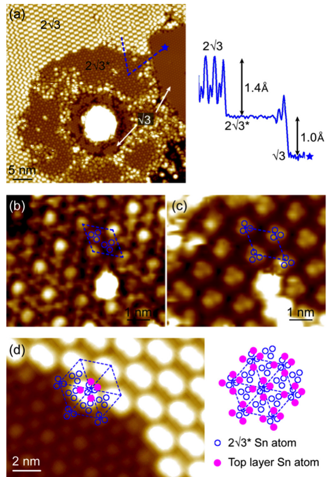
FIG. 2. (a) STM image (+0.8 V, 0.03 nA) of the B- 2\sqrt{3} -Sn surface after applying a +2 V voltage pulse to the STM tip. The large circular area was completely covered with the 2\sqrt{3} -Sn surface before the pulse was applied (image not shown), except for the presence of the native \sqrt{3} -Sn area on the far right of the image. Before pulsing the tip, the tip-sample separation was decreased by about 0.5 nm relative to the normal imaging set point. The bright area below the center of the image likely represents a pile of Sn atoms originating from the top layer of the 2\sqrt{3} reconstruction. Just outside the bright area is a ring of a newly created \sqrt{3} -Sn structure and an unknown 2\sqrt{3}^* phase. The latter is the exposed underlayer of the 2\sqrt{3} -Sn surface. It also has a (2\sqrt{3} \times 2\sqrt{3})R30^\circ periodicity but the structure is different from the 2\sqrt{3} reconstruction. The 2\sqrt{3}^* layer is higher than the neighboring \sqrt{3} structure but lower than the neighboring 2\sqrt{3} structure, indicating that the 2\sqrt{3}^* structure is a single layer structure but with a higher Sn atom density as compared to the \sqrt{3} phase. The line scan illustrates the bilayer nature of the original 2\sqrt{3} reconstruction. Outside the circular 2\sqrt{3}^* region, the native 2\sqrt{3} phase is coexisting with 4\sqrt{3} phase. The latter must be induced by the positively biased pulse or during the scanning process. (b) and (c) are STM images of the same area of the 2\sqrt{3}^* structure, scanned at different tunneling conditions [+0.1 V 0.02 nA for (b); +1.3 V 0.02 nA for (c)], revealing the existence of two downward-pointing trimers and one upward-pointing trimer, indicating a coverage of nine Sn atoms per 2\sqrt{3} unit cell, or 9/12 ML. (d) illustrates the registry of the top layer Sn atoms of the neighboring 2\sqrt{3} domain on top of the 2\sqrt{3}^* underlayer structure. This registry is used as a starting point for the structure refinement in DFT and LEED.
