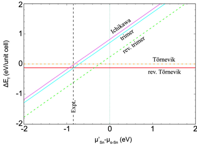
FIG. 5. Formation energies of the candidate structures presented in Fig. 3, calculated as a function of the chemical potential of the Sn adatoms, according to Eq. (1). The chemical potential is determined by the experimental growth conditions and is estimated using Eq. (2) to be -0.85 eV (dashed vertical line).
