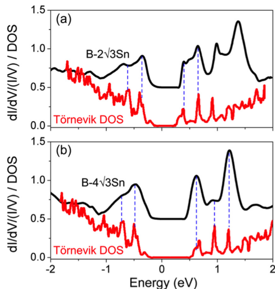
FIG. 14. (a) Line up of the normalized dI/dV spectrum of the B-2\sqrt{3}\text{Sn} surface and the corresponding density of states according to the undoped Törnevik model. The theoretical band gap has been adjusted (spectrum below E_F shifted 0.25 eV toward higher energy; spectrum above E_F shifted 0.15 eV toward lower energy) so as to match the experimental result. (b) same as in (a) but with the experimental spectrum replaced by the normalized dI/dV spectrum of the B-4\sqrt{3}\text{Sn} surface, and showing an improved line-up. Here, the full theoretical spectrum was shifted 0.15 eV toward a higher energy without the artificial band gap correction.
