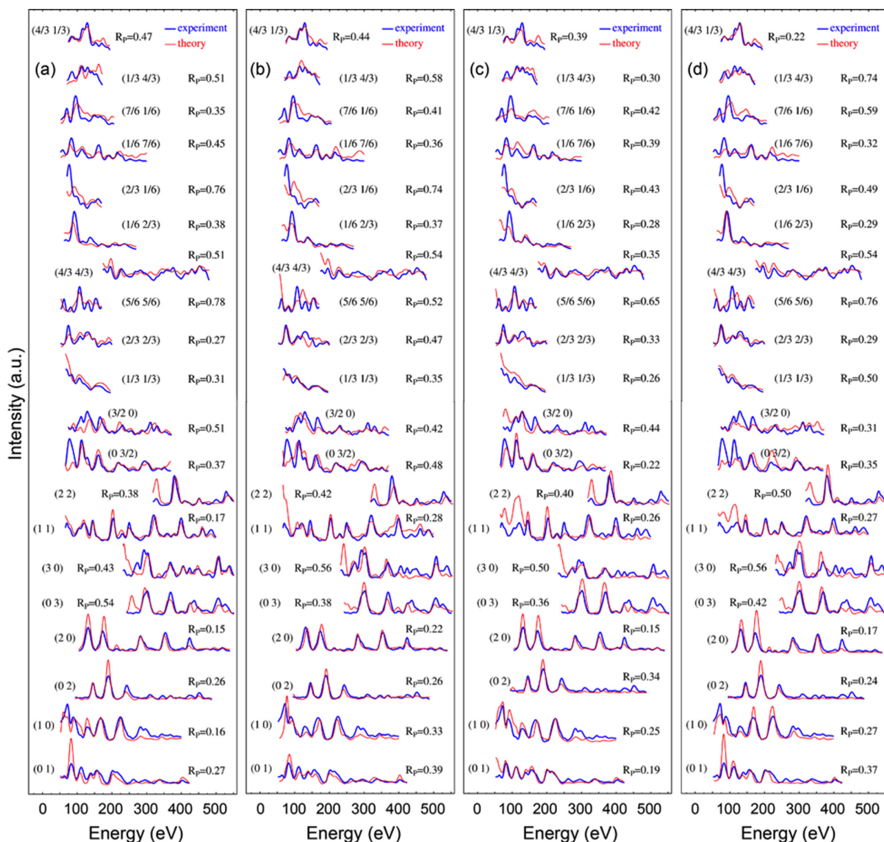
FIG. 7. LEED I - V data of the n-2\sqrt{3}Sn surface, and best fit calculated intensities according to (a) the Törnevik model; (b) revised Törnevik model; (c) trimer model; and (d) revised trimer model. R_p factors for the individual beams are indicated. The overall R_p factors for these models are listed in Table II.
