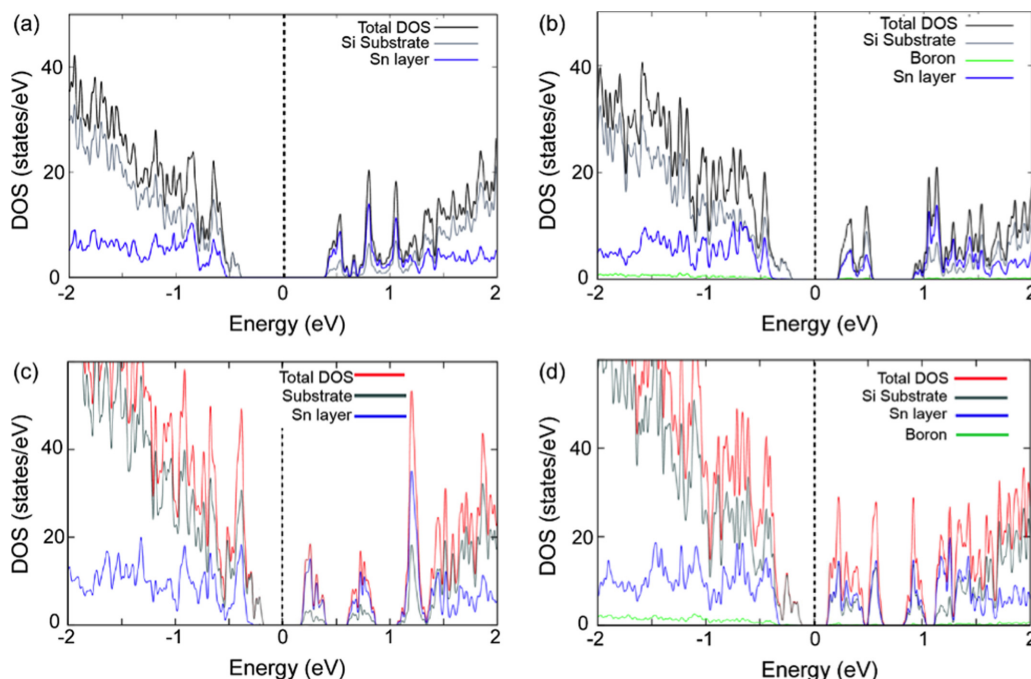
FIG. 13. DFT calculations of the density of states using the HSE functional. (a) and (b) show the density of states for the 2\sqrt{3} Törnevik model, without and with a (\sqrt{3} \times \sqrt{3})R30^\circ boron underlayer, respectively. (c) and (d) show the density of states for the 2\sqrt{3} revised trimer model without and with the (\sqrt{3} \times \sqrt{3})R30^\circ boron underlayer, respectively.
