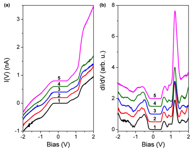
FIG. 17. (a) Raw I(V) and (b) dI/dV spectra of the B- 4\sqrt{3}\text{Sn} surface, measured at 4.4 K. The corresponding normalized dI/dV data are shown in Fig. 12(b).
