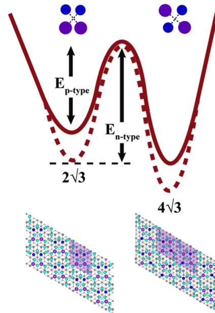
FIG. 16. A possible transition state diagram for the quantum tunneling transition between the 2\sqrt{3} and 4\sqrt{3} structures, where the 4\sqrt{3} structure is assumed to be the most stable configuration for both the n - and p -type samples. The energy diagrams of the electron-doped and hole-doped systems are indicated by the dashed and solid lines, respectively. In this particular case, the barrier for the 2\sqrt{3} to 4\sqrt{3} conversion is the lowest for the p -type system, while the reverse transition remains highly unlikely for both the n -type and the p -type systems. The total-energy minimized structures of the 2\sqrt{3} Sn (left) and 4\sqrt{3} Sn (right) phases are shown for easy comparison.
