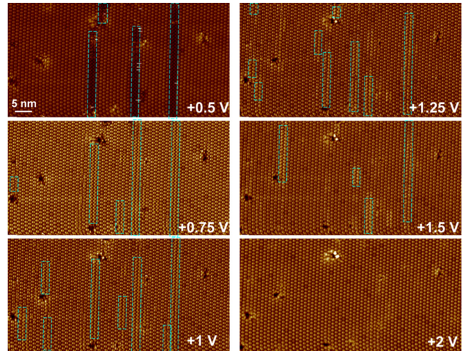
FIG. 15. Bias-dependent STM images of the p - 2\sqrt{3} phase at 77 K. The images are taken on the same area, and with the same tunneling current of 1 nA. The 4\sqrt{3} domains are marked with dashed rectangles. It can be seen that the 4\sqrt{3} fraction reaches a maximum at a scanning bias between 1.00 and 1.25 V.
