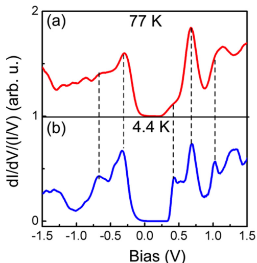
FIG. 10. Line-up of the normalized dI/dV spectra of the B-2\sqrt{3}\text{Sn} surface, recorded at (a) 77 and (b) 4.4 K. The 77-K spectrum was published in Ref. [17]. Both spectra were recorded with the STM tip positioned above an up atom of the B-2\sqrt{3}\text{Sn} structure.
