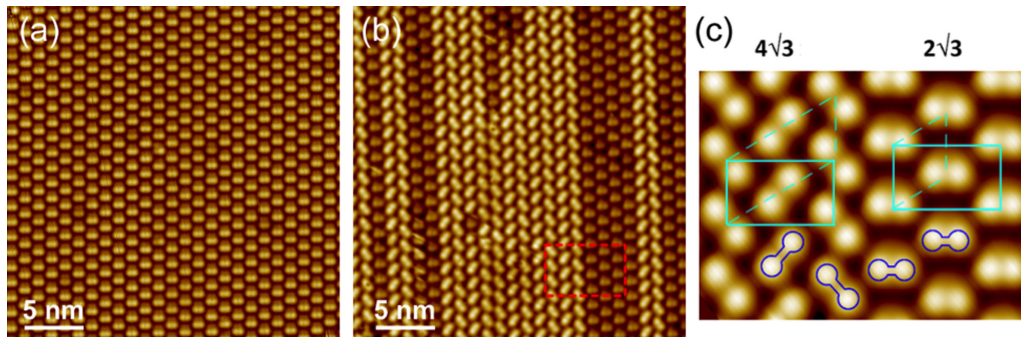
FIG. 1. Scanning tunneling microscopy images of the hole doped \text{Si}(111)(2\sqrt{3} \times 2\sqrt{3})R30^\circ\text{-Sn} interface. (a) shows a uniform 2\sqrt{3} phase at room temperature. The image in (b) shows coexisting 2\sqrt{3} and 4\sqrt{3} domains at 4.4 K. The 2\sqrt{3} to 4\sqrt{3} transition does not occur in the electron-doped system (images not shown; see Ref. [17]). The tunneling parameters are +2 V and 0.1 nA in (a) and +1.5 V, 0.02 nA in (b). (c) shows a close up image (+0.8 V, 0.15 nA) of the surface area marked in (b). Dashed lines mark the primitive (2\sqrt{3} \times 2\sqrt{3})R30^\circ and (4\sqrt{3} \times 2\sqrt{3})R30^\circ unit cells of the 2\sqrt{3}\text{Sn} and 4\sqrt{3}\text{Sn} phases, respectively, while solid lines mark the corresponding centered-rectangular and rectangular unit cells. Up dimers are marked by dumbbells.
