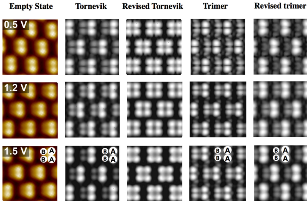
FIG. 9. Experimental (left column) and simulated grayscale STM images for various structure models. The experimental and theoretical images are compared for three different empty state biases, as the lower dimer atoms are not well resolved in filled state images.
