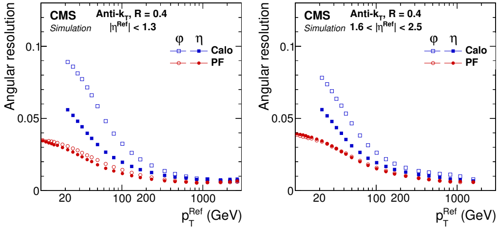
Figure 10. Jet angular resolution in the barrel (left) and endcap (right) regions, as a function of the p_T of the reference jet. The \phi resolution is expressed in radians.
