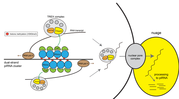
Fig. 1. A model of splicing-independent loading of THO/TREX onto nascent RNAs from a dual-strand piRNA cluster. The RDC complex, which is composed of Rhino, Deadlock (not shown in the figure) and Cuff, is recruited to dual-strand piRNA cluster by recognizing H3K9me3 marks, and facilitates convergent transcription. THO/TREX is loaded onto dual-strand precursor RNAs via interaction of Thoc5 with Cuff. The loading of THO/TREX not only facilitates efficient transcription of precursor RNAs but also mediates their export through nuclear pores into the nuage, a germ-cell specific cytoplasmic structure where piRNA precursors are processed into mature piRNAs.
