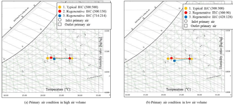
Fig. 7 The temperature changes in primary channel
