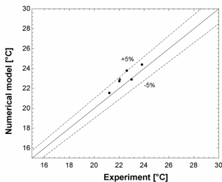
Fig. 6 The primary air outlet temperature of the model and the experiment
