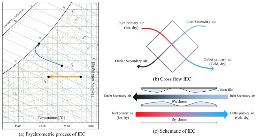
Fig. 1 Cooling process of indirect evaporative cooler
