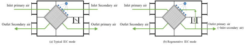
Fig. 3 Two operation modes of IEC
