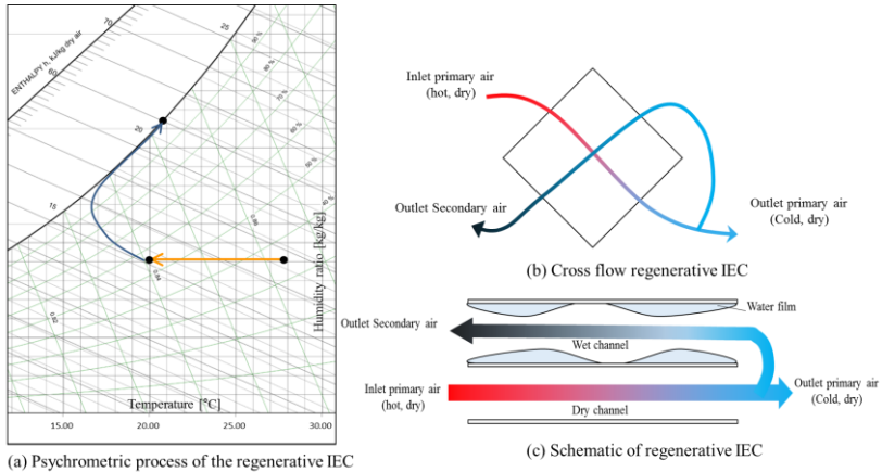
Fig. 2 Cooling process of regenerative indirect evaporative cooler
