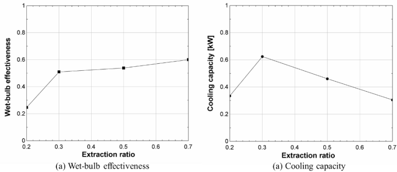
Fig. 5 Effects of extraction ratio in regenerative IEC
