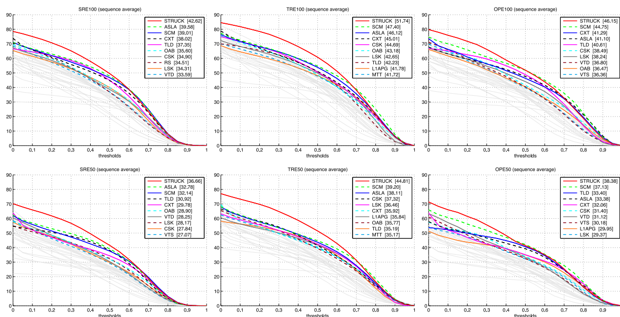
Fig. 4. Plots of OPE, SRE, and TRE on TB-100 (first row) and TB-50 (second row). The score for each tracker is shown in the legend. The top 10 trackers are presented for the sake of clarity, and the rest are shown as gray dashed curves.
