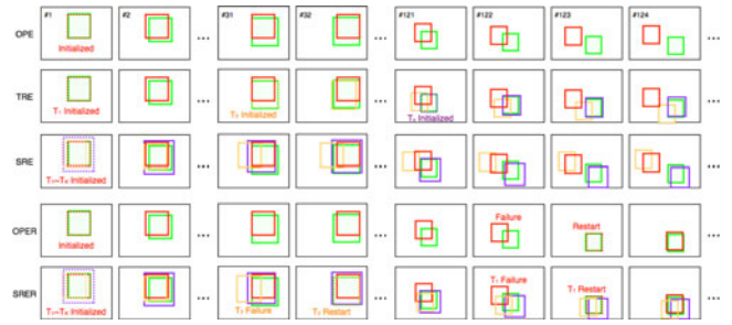
Fig. 2. Evaluation methods for trackers. In each image, the green box represents the ground-truth target location, and the other colors denote the tracker outputs. Dotted boxes represent the initialization of the tracker. OPE is the simplest—initialize the tracker in the first frame and let it track the target until the end of the sequence. In TRE, a tracker starts at different starting frames initialized with the ground-truth bounding box. In SRE, each tracker runs several times with spatially shifted and scaled initializations. The OPER and SRER metrics are used for restarting a tracker for the rest of the sequence if it fails (based on an overlap threshold) at some frame.
