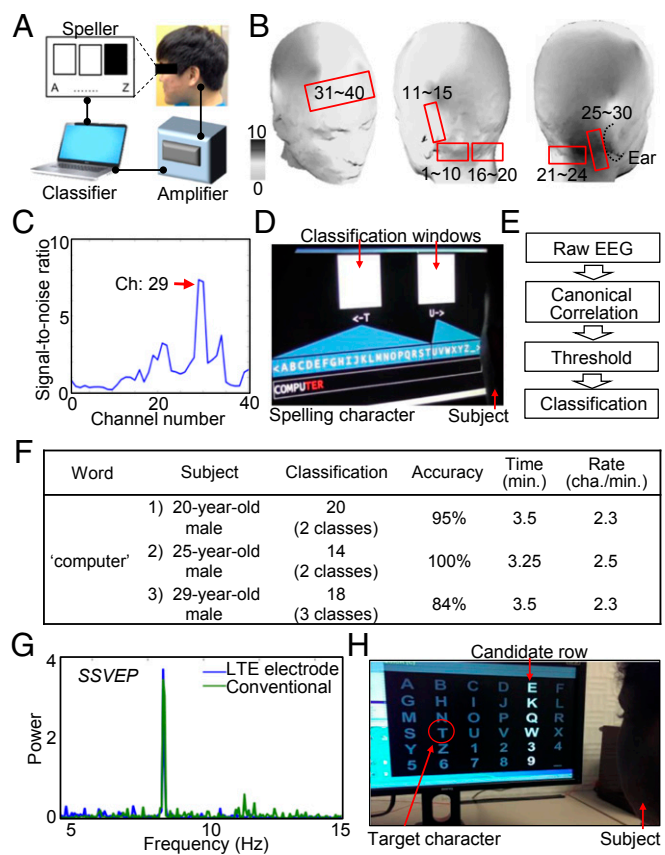
Fig. 5. Recording of steady-state visually evoked potentials (SSVEP) and their use for brain-computer interfaces. (A) Experimental setup for SSVEP-based text speller, showing a visual stimulation, a volunteer wearing electrodes, and a signal amplifier and classifier. (B) Brain mapping with 40 electrodes to identify locations that yield the highest signals. (C) Plot of SSVEP signal quality according to the location. (D) Image of the text speller interface including visual stimulation, classification algorithm, and a volunteer watching the flickering windows. (E) Flowchart of the simplified classification process. (F) Summarized performance of three subjects in the spelling task. The averaged spelling rate for “computer” with word prediction is 2.37 characters/min, and the averaged accuracy is 93%. (G) Comparison of the signals for LTE and conventional gel electrodes. Both exhibit similar patterns and amplitudes. (H) Image of the P300-based text speller to record the event-related potentials to identify the desired letter.
