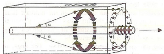
Fig. 2 Mechanical interaction between bar and concrete 10)
