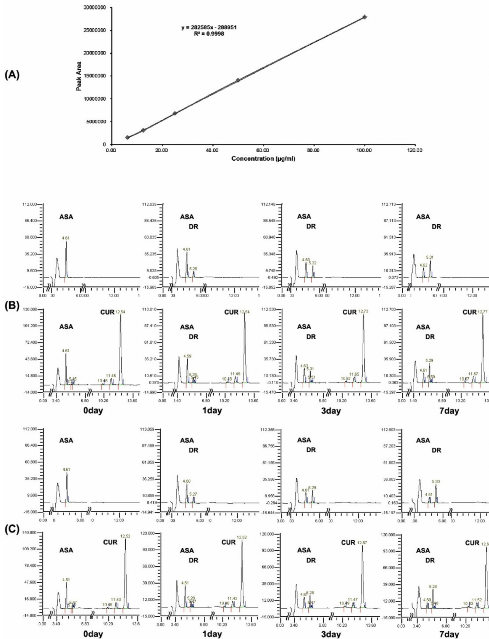
Fig. 1. (A) Calibration curve for the determination of aspirin concentrations (6.25~100 µg/mL). (B) Chromatogram of aspirin(25 µg/mL in DW) and aspirin+curcumin admixture (25 µg/mL+150 µg/mL in DW) and (C) Chromatogram of aspirin(25 µg/mL in NS) and aspirin+curcumin admixture (25 µg/mL+150 µg/mL in NS) after 0, 1 st , 3 rd and 7 th days of storage at 25°C
