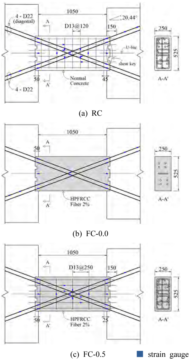
Fig. 2 Reinforcement detail of test specimens (unit: mm)
