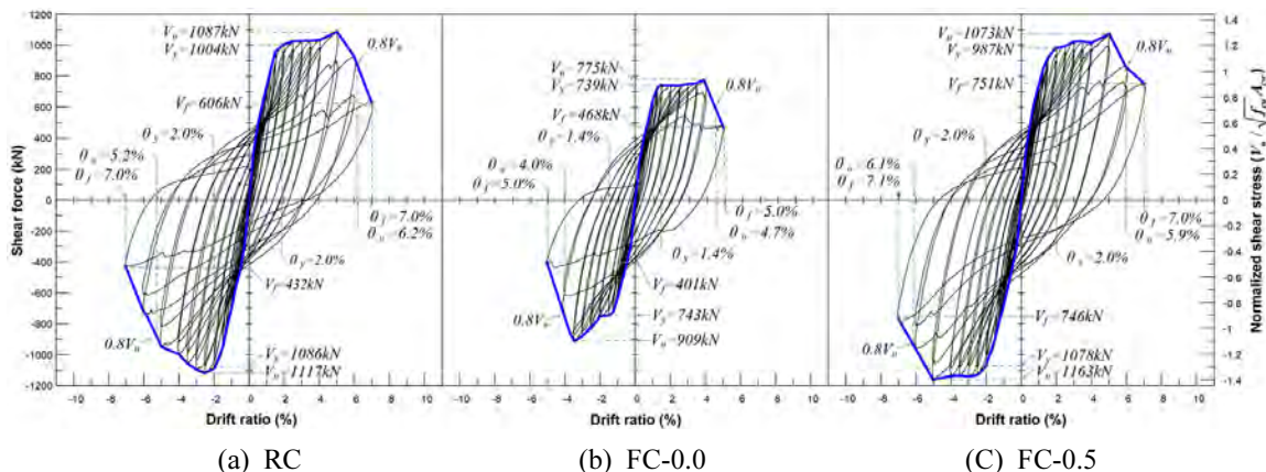
Fig. 6 Lateral force versus drift ratio response
