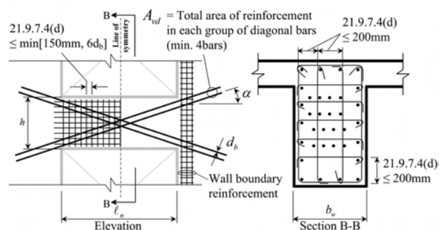
(b) Full confinement of diagonally RC beam section
