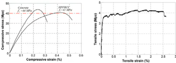
(a) Compressive strength (b) Direct tensile of HPRCC (dog-bone)
