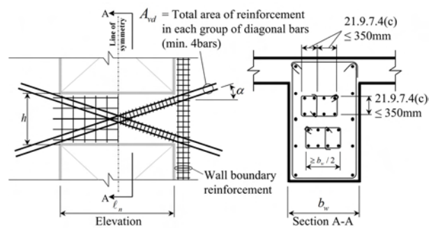
(a) Confinement of individual diagonals
