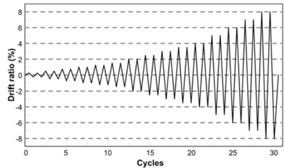
Fig. 4 Loading history
