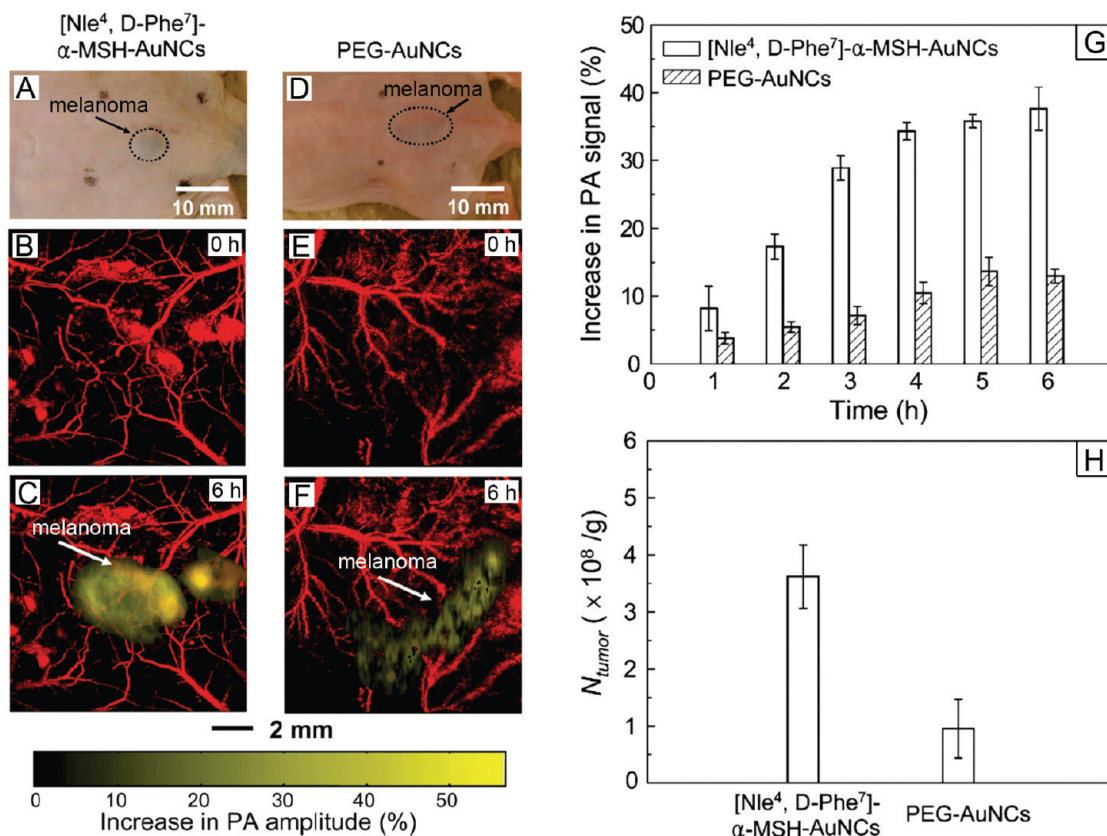
FIGURE 5. (A, D) Photographs of nude mice transplanted with B16 melanomas before the injection of [Nle 4 , D-Phe 7 ]-α-MSH- and PEG-AuNCs, respectively. PA images of the melanoma (B, E) before injection and (C, F) at 6 h postinjection of the two types of AuNCs. (G) Increase of PA amplitude in the melanoma tumors after intravenous injection of the AuNCs ( n = 4 mice for each group) for different periods of time. (H) The average number (per unit tumor mass) of AuNCs accumulated in the melanomas dissected at 6 h postinjection and then measured by ICP-MS. Adapted from ref 22. Copyright 2010 American Chemical Society.
