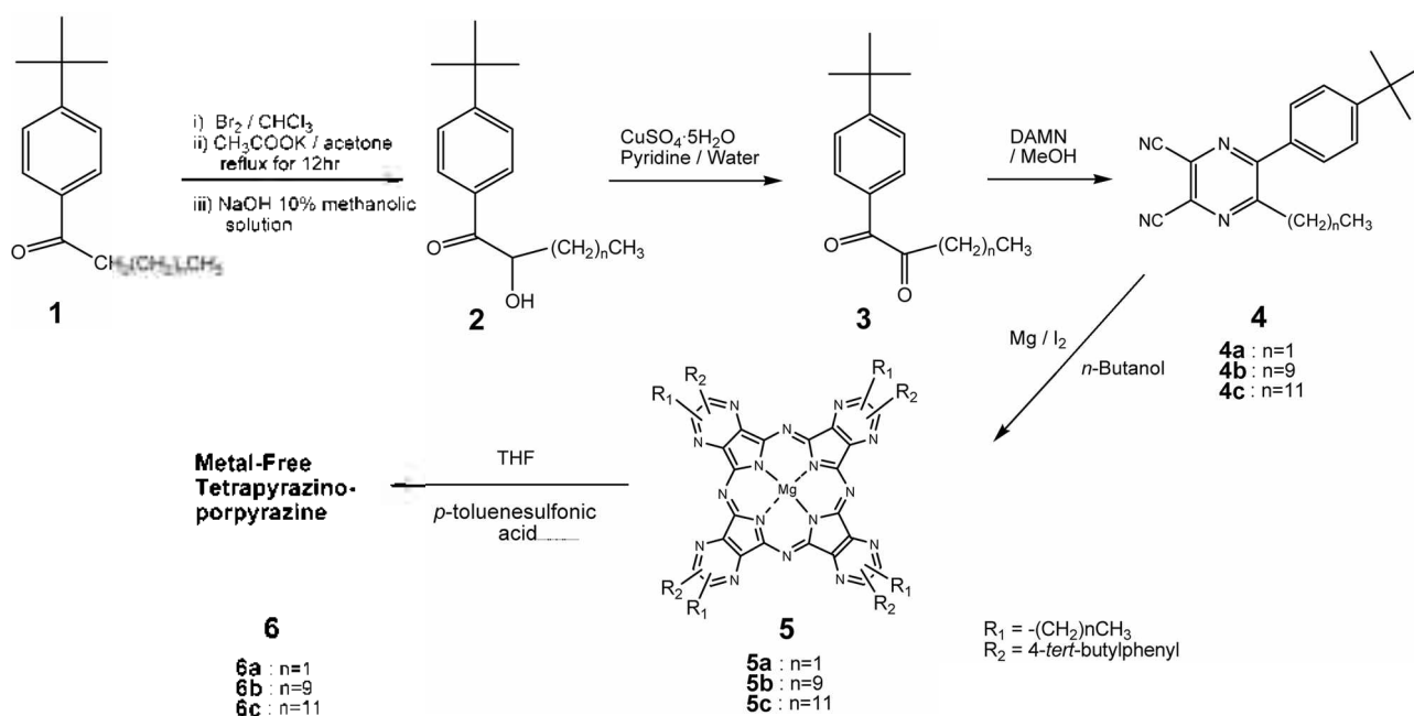
Scheme 1. Synthesis of tetrapyrazinoporphyrazine derivatives.
