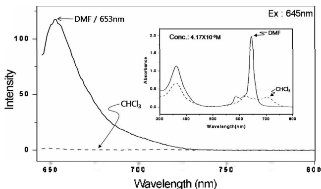
Figure 2. Emission spectra of 5a ( 4.17 \times 10^{-6} M) in DMF and \text{CHCl}_3 .
