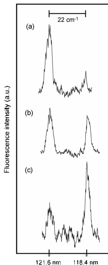
Figure 1. Laser induced fluorescence signal of H and D atoms for (a) CH 3 D, (b) CH 2 D 2 , and (c) CHD 3 .
