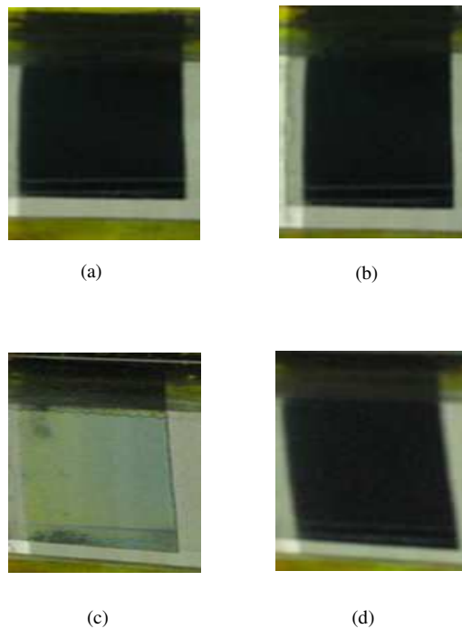
Fig. 5. Photo-images in the dark state of a FFS-TVRL cell; (a) in front view when TVRL is in the nematic phase (20°C), (b) in front view when TVRL is in the isotropic phase (60°C), (c) in side view when TVRL is in the nematic phase (20°C), (d) in side view when TVRL is in the isotropic phase (60°C).
