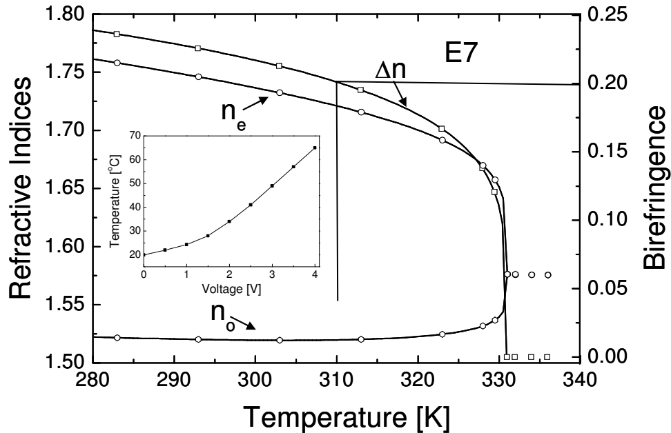
Fig. 2. Temperature-dependent refractive indices and birefringence of E7 LC at wavelength \lambda=560 nm. Squares and circles represent experimental data, and solid lines are fittings using Wu's model.
