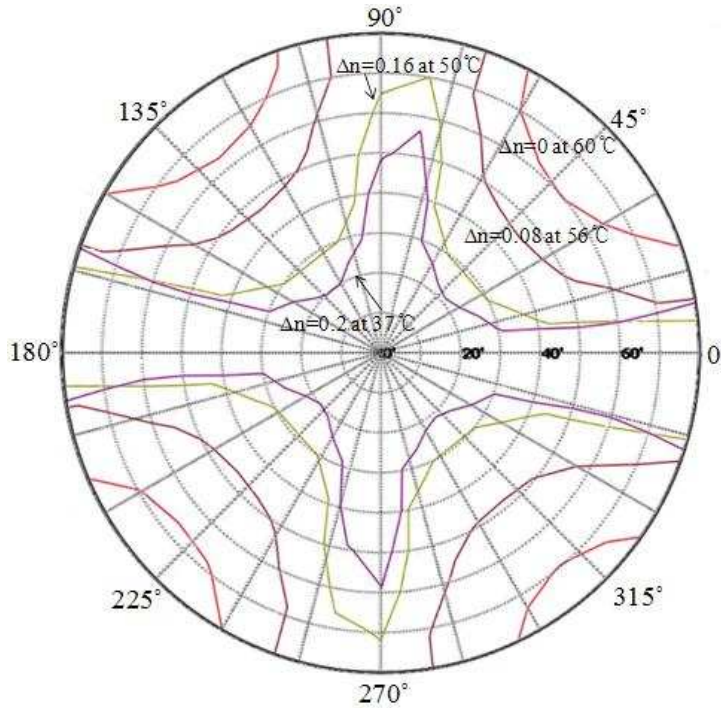
Fig. 3. Simulated results of viewing angle depending on the birefringence of TVRL determined by temperature in the proposed viewing angle controllable FFS mode.
