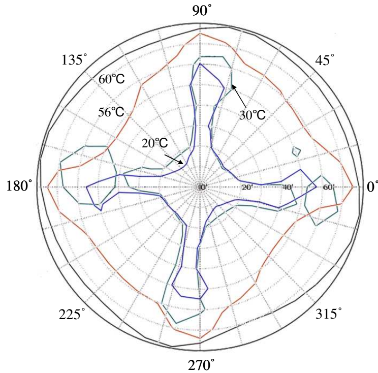
Fig. 4. Measured results of viewing angle according to the temperature of TVRL in the proposed viewing angle controllable FFS mode.
