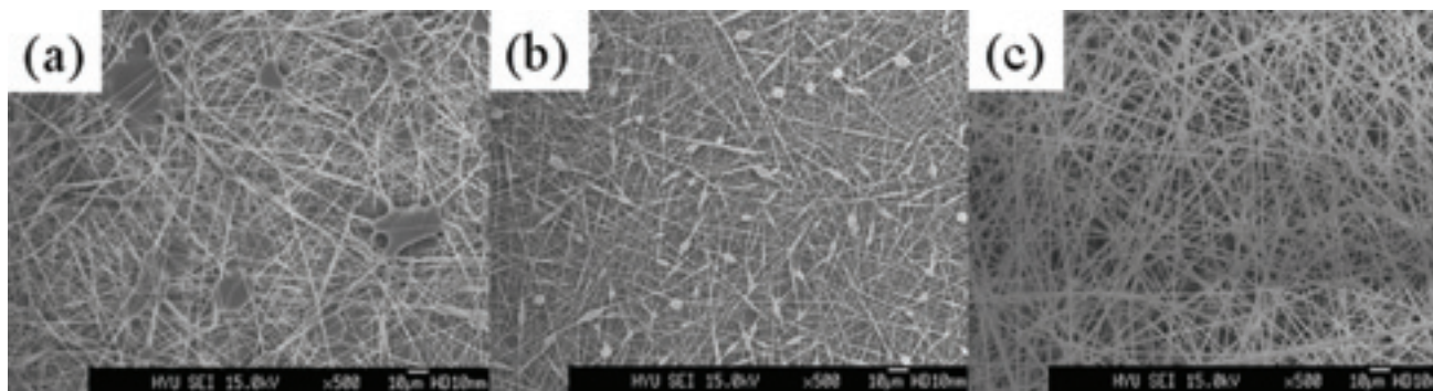
Fig. 2 PES nanofiber web obtained by the electrospinning condition of (a) 40 wt% NMP solution, 25 cm N-C Distance, and 15.9 kV applied voltage ; (b) 35 wt% DMF solution, 25 cm N-C Distance, and 16.7 kV applied voltage ; (c) 37.5wt% DMAc solution, 20 cm N-C Distance, and 15.8 kV applied voltage. Feeding rate was 1.0 ml/h for all.
