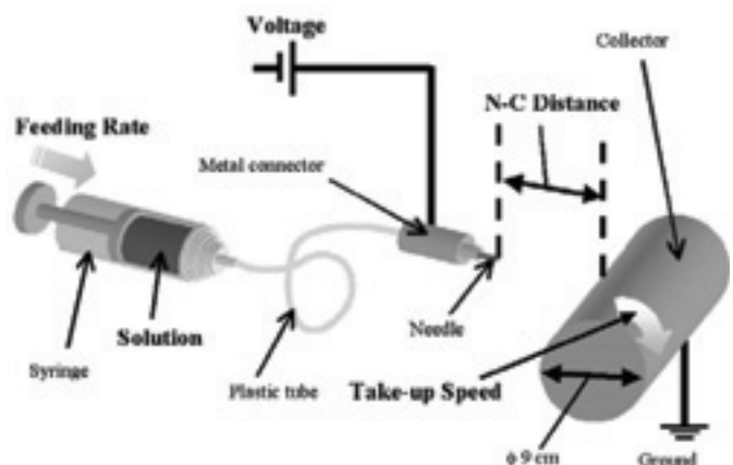
Fig. 1 Schematic diagram of electrospinning system.
