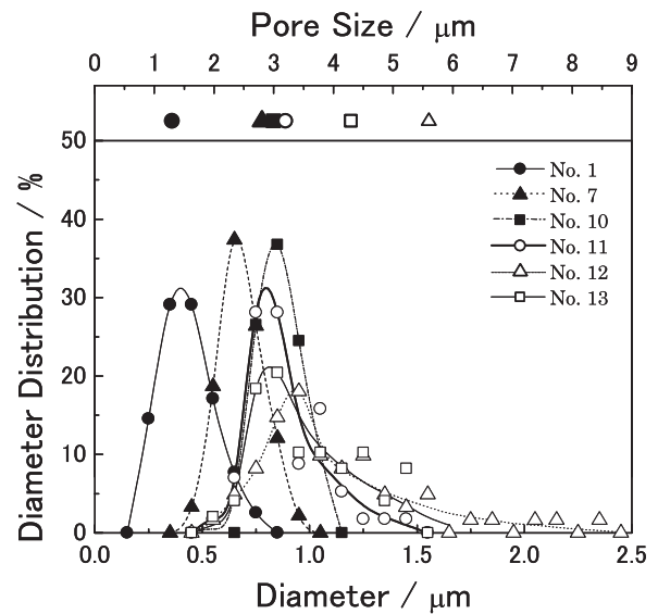
Fig. 6 Fiber diameter and Pore size of the PES web. Electrosinning conditions are corresponding to No.1, No.7, No.10, No.11, No.12, and No.13 of Table 2.
