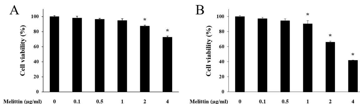
Figure 1. Cytotoxicity of melittin in HaCaT cells. HaCaT cells were treated with different concentrations of melittin for 8 h (A) and 24 h (B). Results are expressed as the mean \pm SEM of three independent determinations. * p < 0.05 compared to the untreated group.
