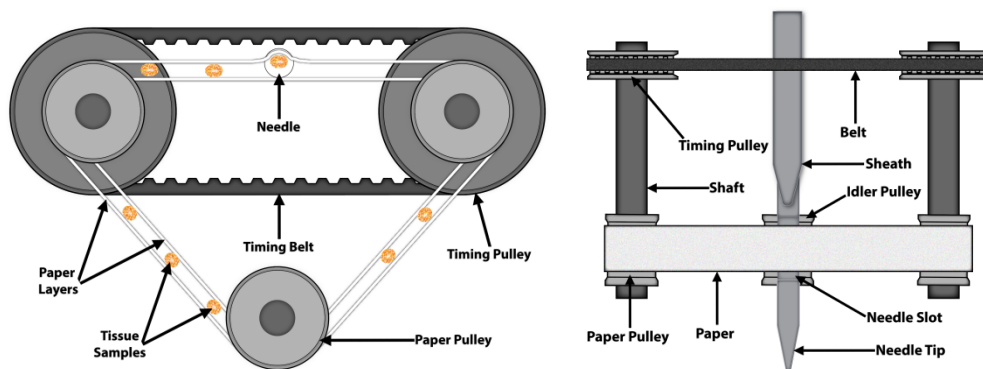
FIGURE 3. Schematic of working principle of MTSCD: front view (Left), top view (Right)
