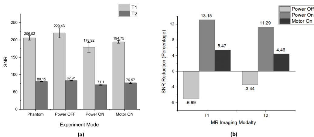
FIGURE 11. MRI compatibility evaluation test results: (a) SNR plotted for T1 and T2 imaging modalities against 04 testing configurations (b) SNR reduction in percentage plotted against T1 and T2 imaging modalities for 03 testing configurations
