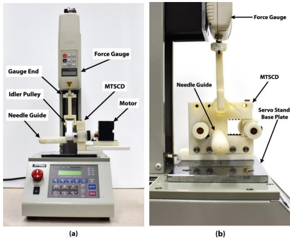
FIGURE 6. Parameters optimization experimental setup: (a) Side View (b) Front View
