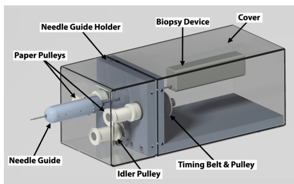
FIGURE 2. Multiple tissue sample collection device (MTSCD): 3D model (Left), 3D printed prototype (Right)
