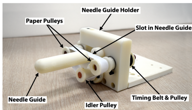
FIGURE 2. Multiple tissue sample collection device (MTSCD): 3D model (Left), 3D printed prototype (Right)
