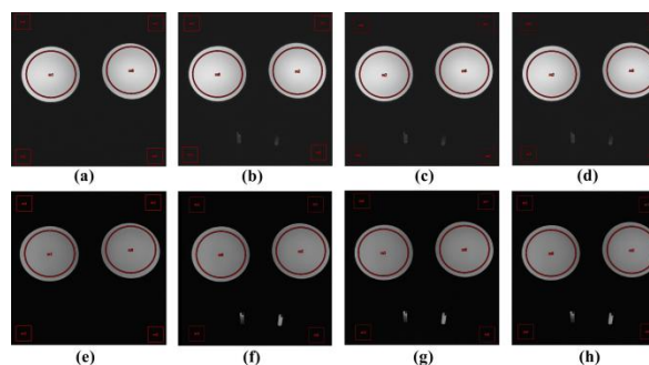
FIGURE 10. MRI scans: (a),(e) Phantom only, (b), (f) MTSCD placed in the bore with power off (c), (g) MTSCD placed in the bore with power on (d),(h) MTSCD placed in the bore while motor is operational. The upper image series (a)-(d) is T1 weighted while and the lower image series (e)-(d) is T2 weighted.
