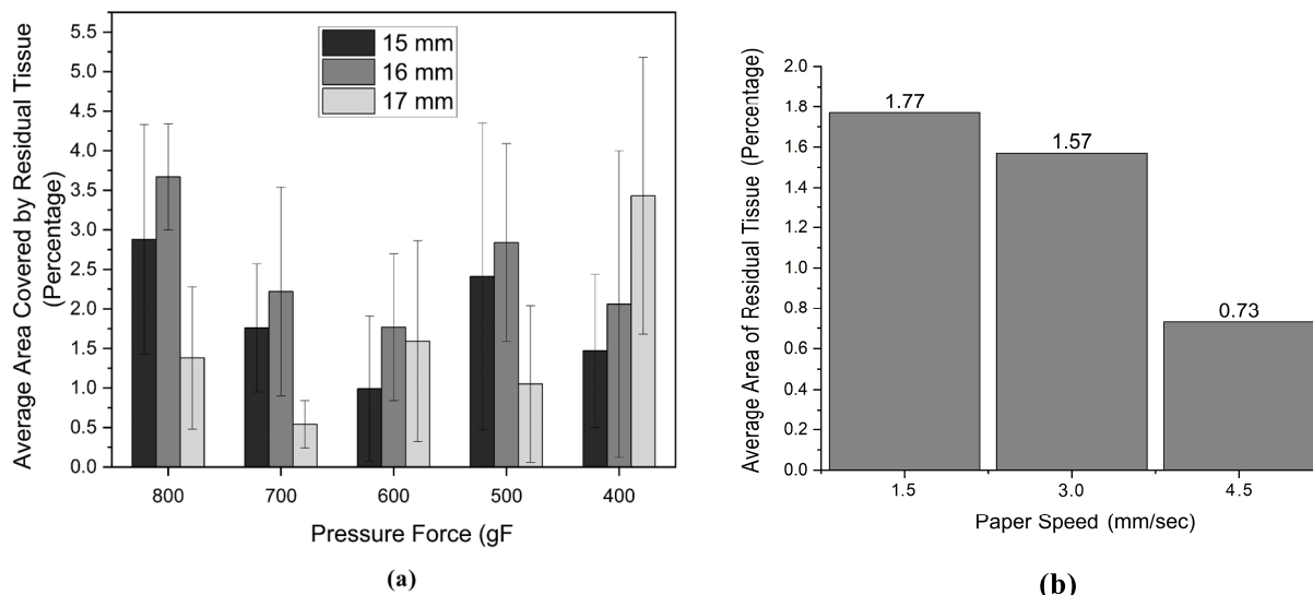
FIGURE 8. Optimization Results: (a) Residual tissue percentage plotted against pressure force for different widths of paper (b) Residual tissue percentage plotted against speed of the motor.
