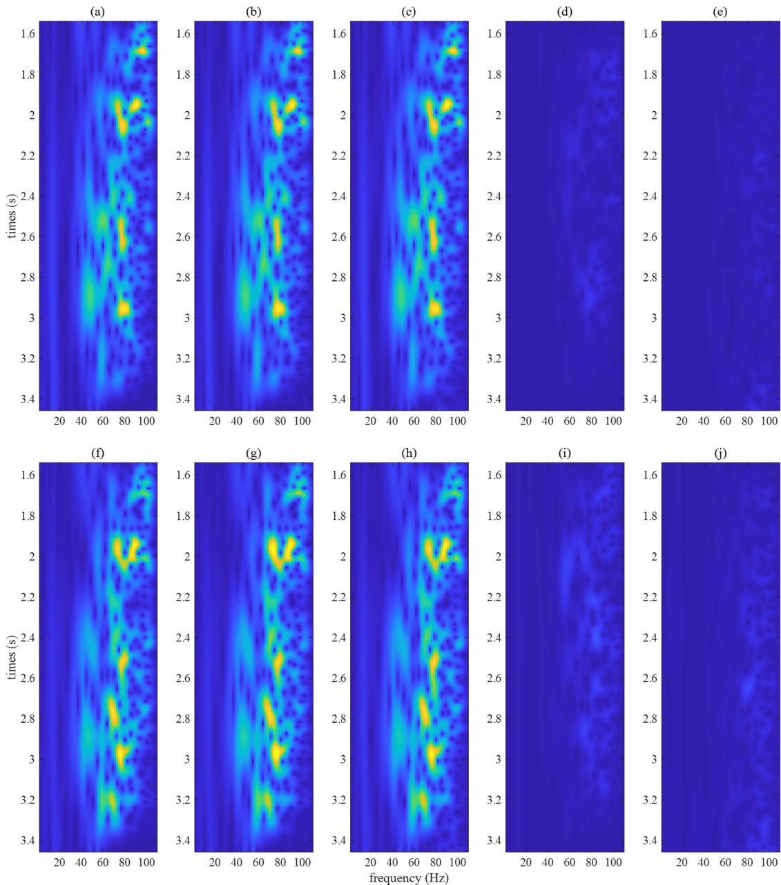
Fig. 10. Scalograms using continuous wavelet transform (CWT) at XL = 16.65 (a-e) and 16.85 (f-j) locations in Fig. 3b. (a, f) Ground truth. (b, g) Prediction using the proposed method. (c, h) Prediction using the MWNI method. (d, i) Difference between ground truth and prediction using the proposed method. (e, j) Difference between ground truth and prediction using the MWNI method.
