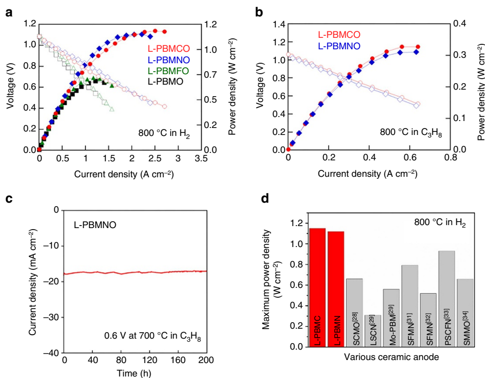
Figure 4 | Electrochemical properties of layered \text{PrBaMn}_{1.7}\text{T}_{0.3}\text{O}_{5+\delta} anode in fuel cells. (a) I - V curve and the corresponding power densities of the L-PBMT0 (T = Mn, Co, Ni and Fe) electrode using humidified (3% \text{H}_2\text{O} ) \text{H}_2 and ambient air as the oxidant at 800 °C. (b) I - V curve and the corresponding power densities of the \text{PrBaMn}_{1.7}\text{Co}_{0.3}\text{O}_{5+\delta} (L-PBMCO) and \text{PrBaMn}_{1.7}\text{Ni}_{0.3}\text{O}_{5+\delta} (L-PBMNO) electrode using \text{C}_3\text{H}_8 as fuel and ambient air as the oxidant at 800 °C. (c) Electrochemical performances of L-PBMNO anode in \text{C}_3\text{H}_8 at 700 °C under a constant voltage of 0.6 V. (d) Comparison of the maximum power density at 800 °C in \text{H}_2 of the present work and other studies in the literature 28–34 .
