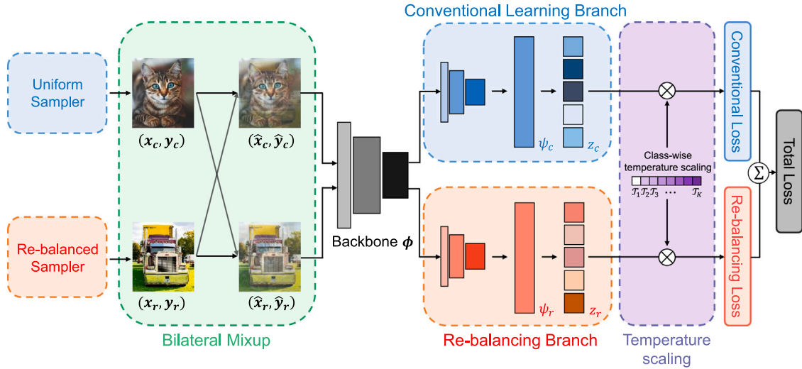
Fig. 2. Overview of the proposed method: Our method use two bilateral mixup samples (\hat{x}_c, \hat{y}_c) and (\hat{x}_r, \hat{y}_r) to train two branch networks, conventional learning branch and re-balancing branch. In the training phase, we use (\hat{x}_c, \hat{y}_c) for conventional learning branch and (\hat{x}_r, \hat{y}_r) for re-balancing branch. For the inference phase, two prediction logits from each branch are averaged to return the final output.
