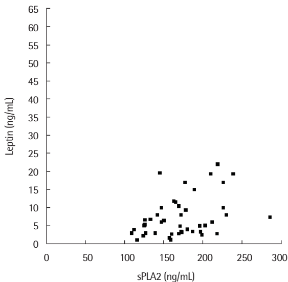
Fig. 2. Secreted phospholipase A2 (sPLA2) levels were significantly correlated with serum leptin levels in asthmatic subjects (n=46, r=0.318, P=0.033). r, partial correlation coefficient adjusted for body mass index.
