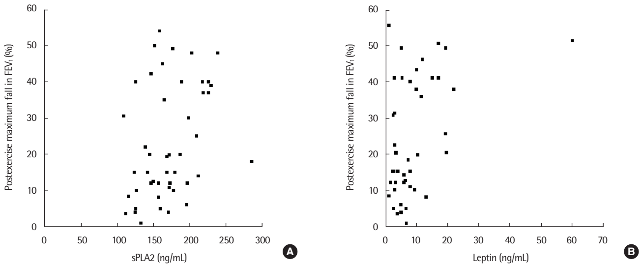
Fig. 3. The maximum decreases in % forced expiratory volume in 1 second (FEV 1 ) after exercise were significantly correlated with both phospholipase A2 levels (A: n=46, r=0.301 , P=0.041 ) and leptin levels (B: n=46, r=0.346 , P=0.018 ). r , partial correlation coefficient adjusted for body mass index.
