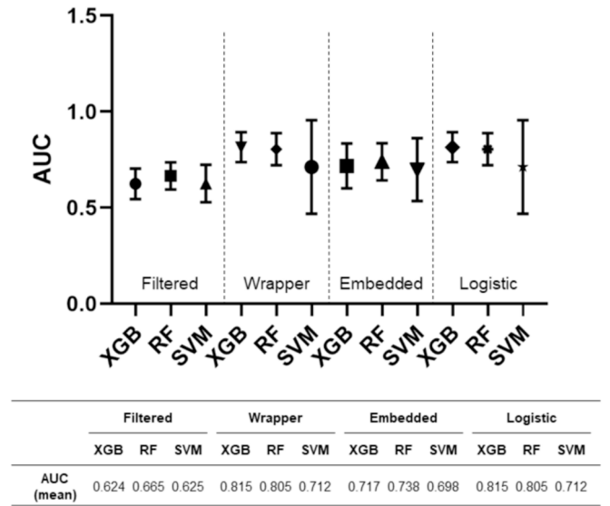
Fig. 2. The predictive performance (area under the curve (AUC): mean ± standard deviation) of the different combinations of feature selection methods and machine learning models, as evaluated through repeated nested cross-validation with SMOTE.
