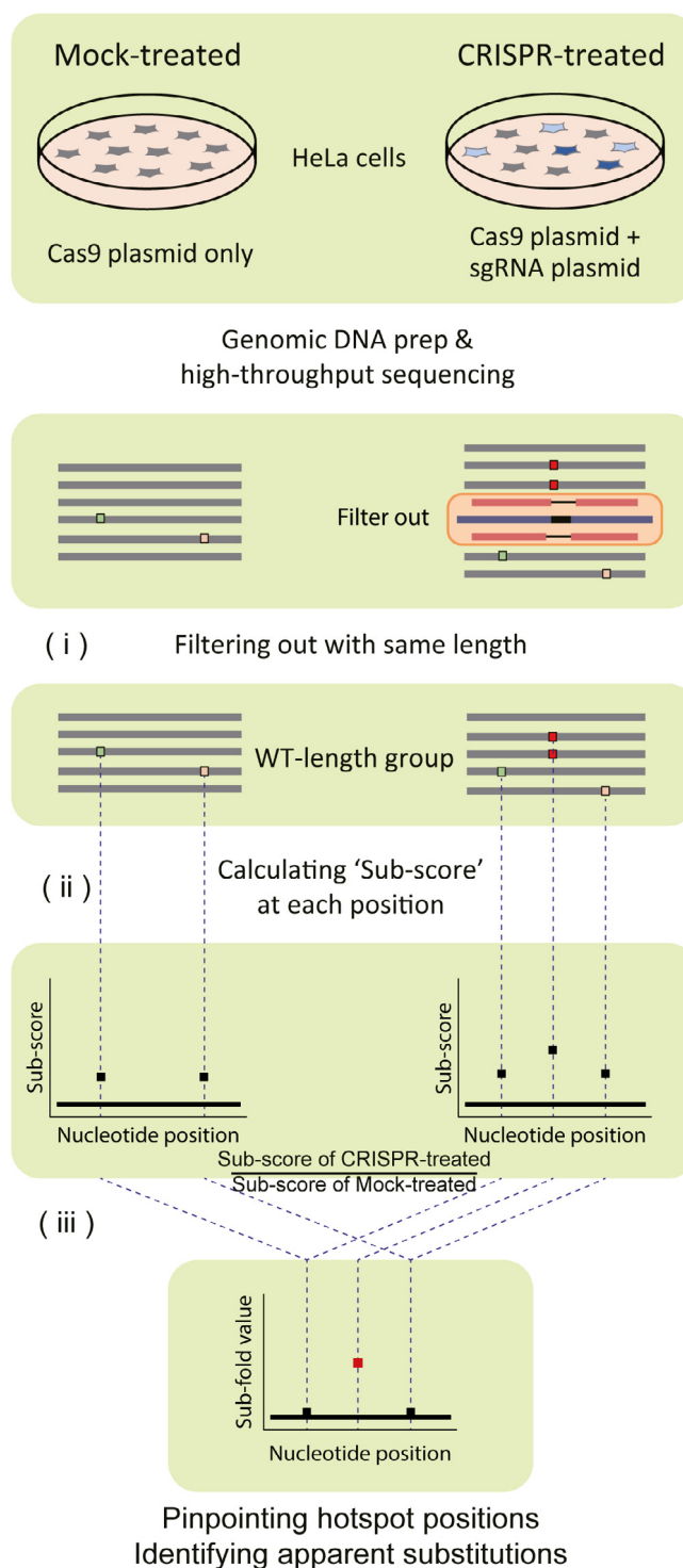
Fig. 1. Scheme of the CRISPR-Sub analysis platform. Mock-treated HeLa cells are treated only with a plasmid encoding SpCas9, whereas CRISPR-treated HeLa cells are treated with plasmids encoding SpCas9 and sgRNA. Genomic DNA is extracted from both Mock- and CRISPR-treated cells, amplified by targeted deep-sequencing, and analyzed by NGS. Sequences in the WT-length group are collected by filtering out the reads having a length different from that of WT. Sub-scores at each position are calculated by dividing the total number of substitutions at each position by the total number of WT-length queries. To exclude NGS and PCR error signals, the Sub-fold value is calculated by dividing the Sub-score of the CRISPR-treated data by that of the Mock-treated data.
