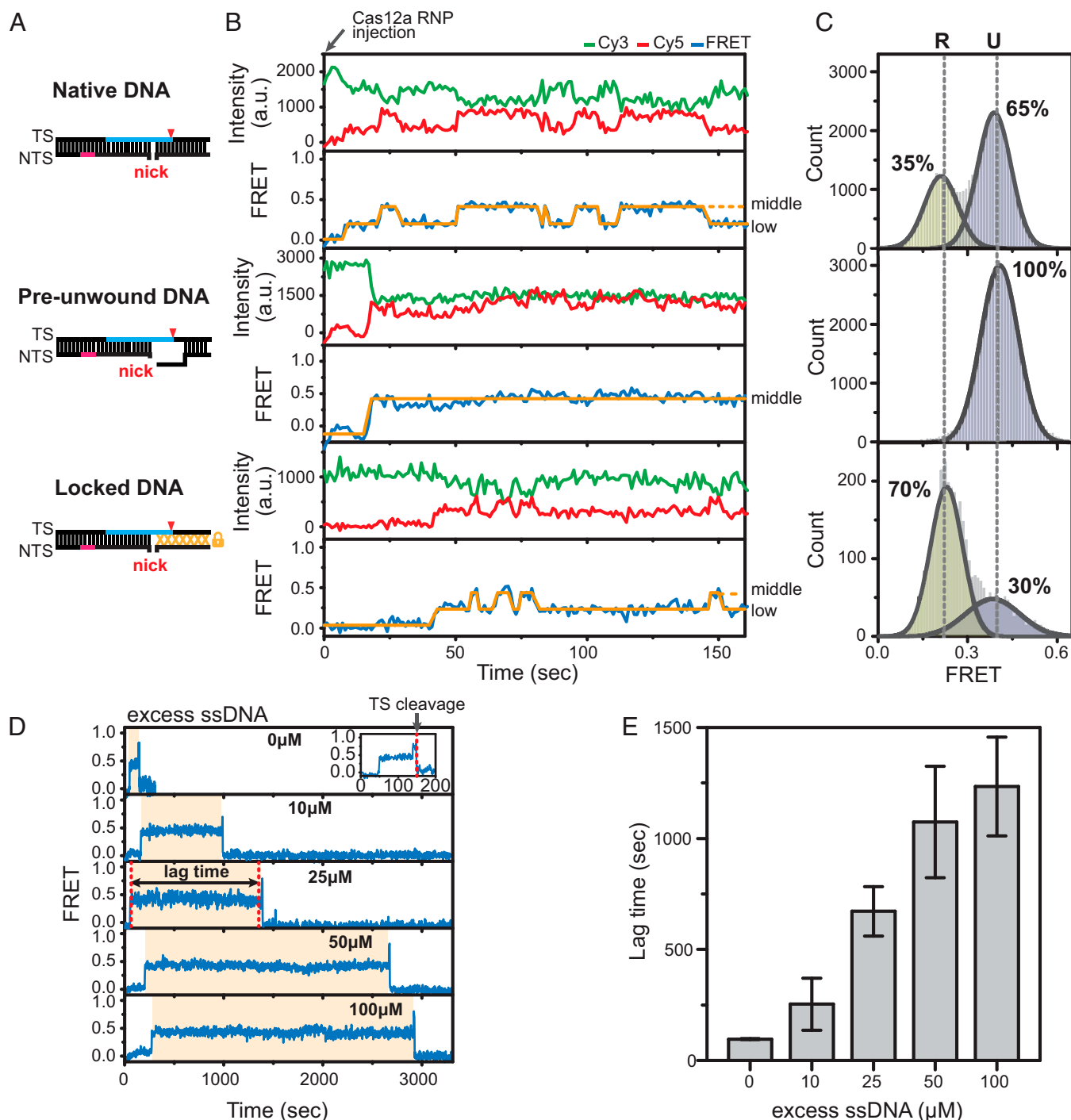
Fig. 2. Defining conformational intermediates in the TS cleavage reaction. (A) NTS prenick DNA constructs (native DNA, Top ; preunwound DNA, Middle ; locked DNA, Bottom ) used for the experiments to assign the FRET states to functional intermediates. (B and C) Representative intensity and FRET time traces showing conformational dynamics of the Cas12a–crRNA–DNA complex in the TS cleavage reaction (B) and corresponding FRET histograms of the Cas12a ternary complex (C) for three NTS prenick DNA constructs (native DNA, Top ; preunwound DNA, Middle ; locked DNA, Bottom ) in the presence of 20 nM Cas12a RNP and 0.5 mM Mg^{2+} . FRET histograms were obtained by collecting all data points for each DNA construct from at least more than 70 time traces. The relative population of each FRET intermediate was obtained by fitting the FRET histogram to the sum of two Gaussian functions. (D) Representative FRET time traces in the presence of 20 nM Cas12a RNP, 10 mM Mg^{2+} , and excess 13-nt single-stranded DNA (ssDNA) substrate with varying concentrations. (E) Lag times of transitions to the high FRET state in the absence and presence of excess 13-nt ssDNA substrate with varying concentrations (10, 25, 50, and 100 \mu M). The lag times were obtained by fitting the data to a single exponential decay function. The error bars in E were obtained from at least more than two independent experiments.
