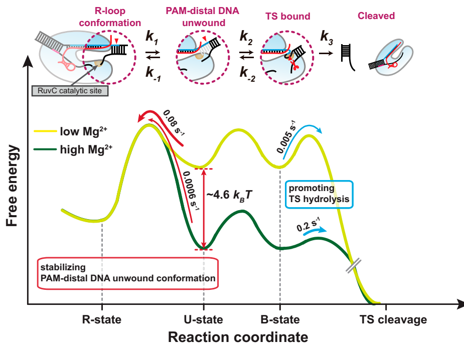
Fig. 4. Proposed model for \text{Mg}^{2+} -dependent conformational rearrangements in the TS cleavage reaction by Cas12a RNP. Cartoon free energy landscapes for the Cas12a–crRNA–DNA complex during the TS cleavage reaction at high (dark green line, 5 mM) and low (light green line, 1 mM) \text{Mg}^{2+} ion concentrations were estimated based on the experimentally determined rate constants for all possible transitions in the TS cleavage reaction. A detailed description of the estimation method is provided in Materials and Methods . The energy barrier for the PAM-distal DNA rewinding is raised by an increase in \text{Mg}^{2+} concentration, and that for the TS cleavage step is lowered by an increase in \text{Mg}^{2+} concentration.
