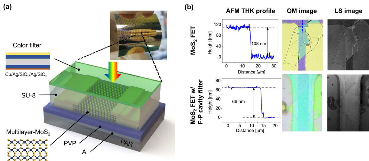
Figure 1. (a) Schematic illustration of the fabricated MoS 2 phototransistor integrated with Fabry-Perot cavity filter and photograph image of the bent device on a PAR substrate. (b) The measured thickness of MoS 2 flakes by atomic force microscope (AFM), optical microscope (OM), and laser scanning (LS) images of a bare MoS 2 phototransistor (bare-MoS 2 ) and MoS 2 phototransistor with F-P cavity filter for amber color are shown on the top-row and on the bottom-row, respectively. The atomic layer numbers corresponding to the MoS 2 thickness were about 166 and 102 layers, respectively, assuming monolayer thickness of 6.5 Å.
