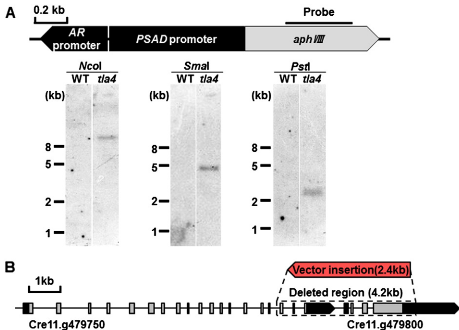
Fig. 4. Genomic DNA organization of the tla4 mutant. A , Southern blot analysis. Genomic DNA was digested with NcoI , SmaI , or PstI . A partial sequence of the aphVIII gene was used as a probe. B , Map of the insertion site in the genomic DNA. The areas marked with a broken line are nucleotides deleted in the tla4 mutant, including a CpSRP54 homolog ( g479750 ) and a portion of the g479800 gene. The red box indicates the plasmid inserted in the deleted region. Arrows indicate the direction of the insertions. Black: untranslated regions. Gray: exons. Horizontal lines: introns.
