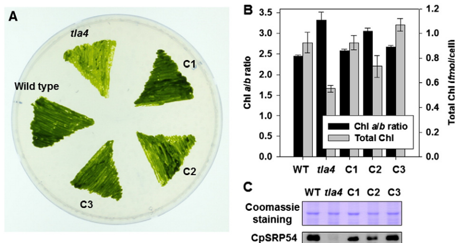
Fig. 5. A , Colonies of wild-type (WT) C. reinhardtii CC-4349 (parental strain of tla4 ), the tla4 mutant, and complemented tla4 lines (C1–C3) under photoautotrophic growth conditions. B , Chl a/b ratios of the above strains ( n = 3 ; values shown are means \pm SD). C , Western blot analysis of total protein extracts from the C. reinhardtii wild type (WT), the tla4 mutant and the tla4 complemented lines C2 and C3. Upper image shows the corresponding SDS-PAGE Coomassie-stained gel.
