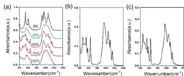
Figure 9. ATR-FTIR spectra of (a) a set of LiNiPO 4 prepared using 0 to 100% of LiH 2 PO 4 (top to bottom), (b) o -LiCoPO 4 , and (c) o -LiMnPO 4 .
