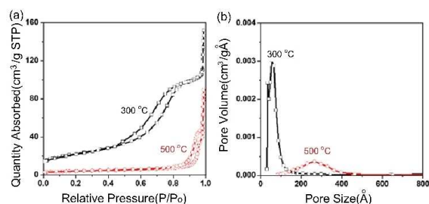
Figure 5. (a) \text{N}_2 adsorption-desorption isotherms of DNI60-300 and DNI60-500 and (b) their BJH pore-size distribution plots.
