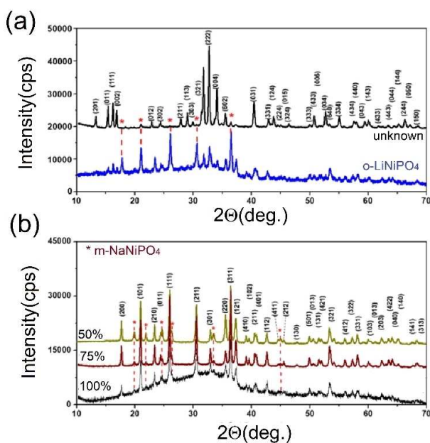
Figure 7. PXRD patterns of \text{LiNiPO}_4 , prepared using (a) 0 and 25% and (b) 50, 75, and 100% \text{LiH}_2\text{PO}_4 (top to bottom) as lithium and phosphate source at 500^\circ\text{C} .
