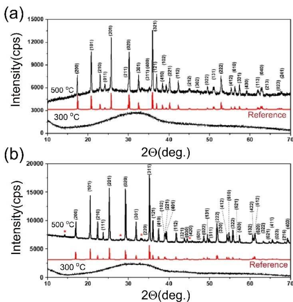
Figure 6. PXRD patterns of calcined (a) \text{LiCoPO}_4 and (b) \text{LiMnPO}_4 at 300^\circ\text{C} (bottom) and annealed to 500^\circ\text{C} (top) and middle ones are reference data.
