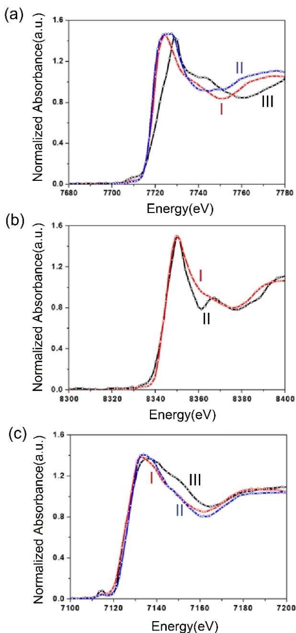
Figure 10. K-edge XANES spectra of LMPs: (a) I) 300 °C and II) 500 °C of LCoP and III) Co 3 O 4 , (b) I) LNiP and II) NiO, and (c) I) 200 °C and II) 500 °C LFeP and III) FePO 4 .
