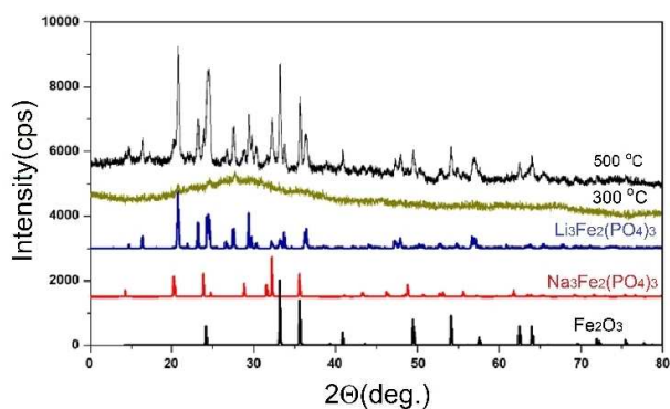
Figure 8. PXRD pattern of DLFeP60, calcined at (a) 300 °C and (b) 500 °C, with PDF data of Fe 2 O 3 , Li 3 Fe 2 (PO 4 ) 3 , and Na 3 Fe 2 (PO 4 ) 3 .
