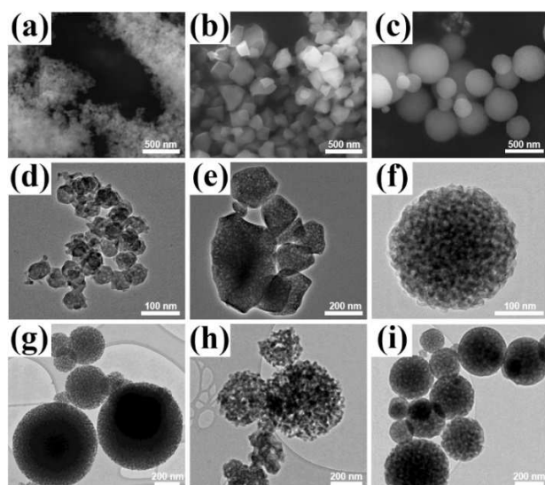
Figure 4. SEM (a-c) and TEM (d-f) images of \text{LiCoPO}_4 , obtained from DLCoP10, DLCoP40, and DLCoP90 and TEM images of (g) \text{LiNiPO}_4 , (h) \text{LiMnPO}_4 , and (i) \text{LiCoPO}_4 .
