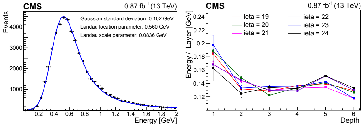
Figure 36. Left: energy deposit from muons in pp collision events in the HE tower corresponding to \eta = 20 and depth = 5. The energy spectrum is fitted using the convolution of a Gaussian function with a mean of zero and a Landau distribution. The fitting function has three free parameters: the Landau location parameter, the Landau scale parameter, and the width of the Gaussian. Right: the most probable value of the muon energy deposit per layer in HE towers as a function of depth for different \eta regions. The vertical bars represent the statistical uncertainty. Muons from collision events are considered when their trajectory is contained within a single HCAL tower. The muon signal peak is fitted with the convolution of a Gaussian and Landau functions. The Landau location parameter is divided by the number of scintillator layers in the considered depth.
