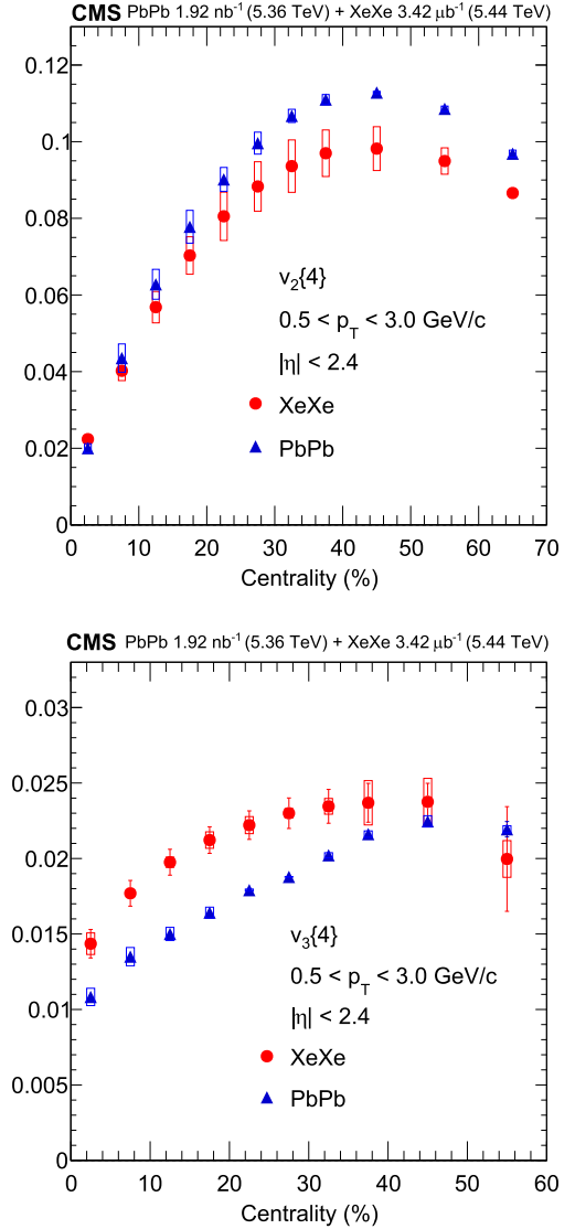
Fig. A.7. Measured v_2\{4\} (upper) and v_3\{4\} (lower) cumulant values as a function of centrality for XeXe and PbPb collisions, calculated using 4-particle cumulants. The vertical bars and open boxes represent the statistical and systematic uncertainties, respectively.
