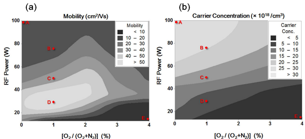
Figure 1. Contour plots of (a) Hall mobility and (b) carrier concentrations of ZnON films, with respect to the RF power and O_2/(O_2 + N_2) ratio. Note that the carrier concentration exhibits a clear trend, while an optimum region exists for the electron mobility.
