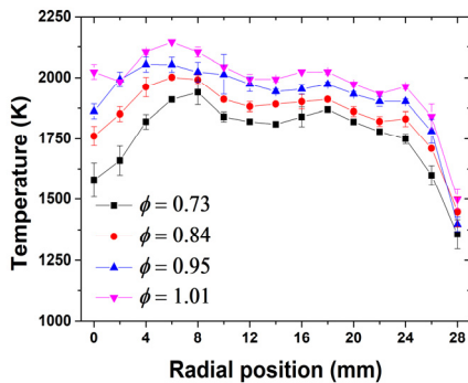
Fig. 10. Radial temperature profiles obtained based on LIBS data and TDLAS data on the spectral line at 7185.6 cm -1 .
