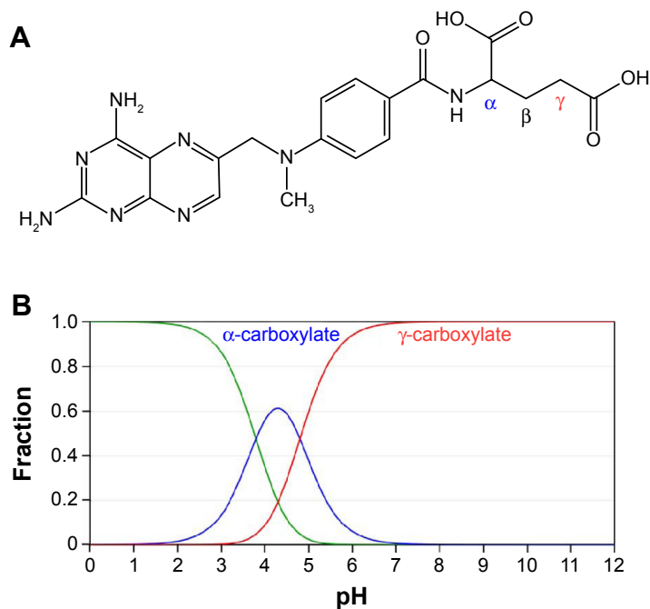
Figure S1 (A) Molecular structure of methotrexate (MTX; (2S)-2-[(4-[[[2,4-diamino-7,8-dihydropteridin-6-yl)methyl]](methyl)amino]phenyl)formamido]pentanedioic acid), and (B) plots of MTX molar fractions vs pH ( pK_{a1}=3.8 , pK_{a2}=4.8 ). 1
