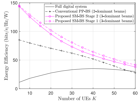
FIGURE 8. Energy efficiency as a function of the number of UEs K . Fixed parameters: N = 81 , L = 0 .
