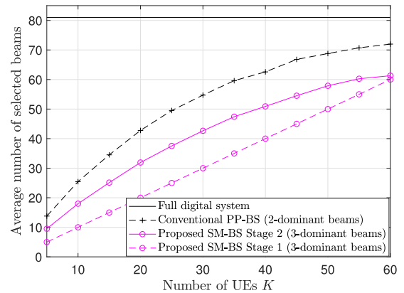
FIGURE 6. Average number of beams (RF chains) used for transmission versus number of UEs K . Fixed parameters: N = 81, L = 0 .
