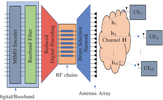
FIGURE 2. Example of beamspace MIMO system architecture.
