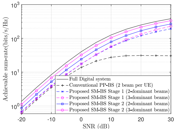
FIGURE 5. Comparison of the achievable sum-rate as a function of SNR (dB) for the proposed beam selection and the conventional projected-power based beam selection. Fixed parameters: N = 81, K = 40, L = 2 .
